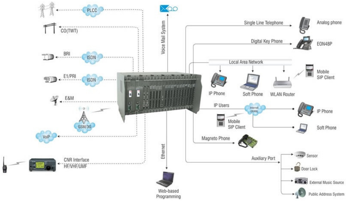
Trunk-side Interfaces
