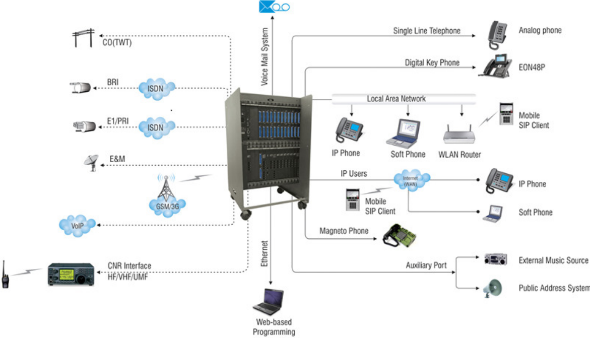
Trunk-side Interfaces
